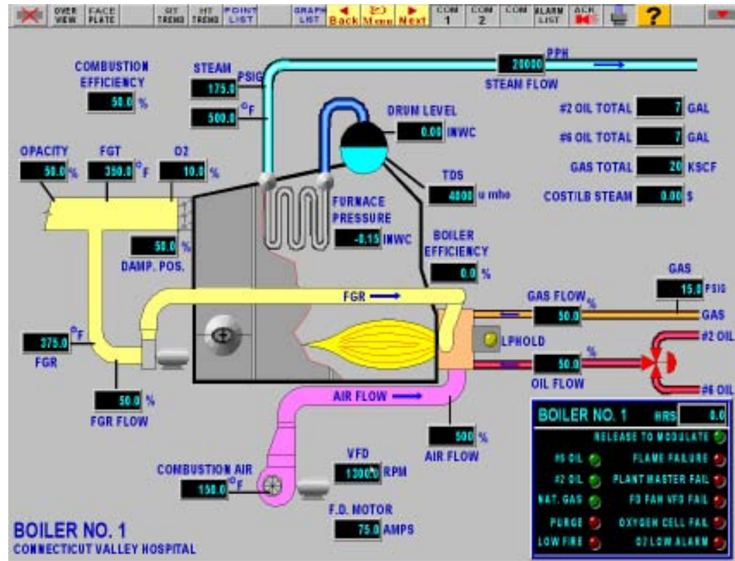
Graphical User Interface: typical SCADA screens. Above, BOILER OPERATION OVERVIEW . Below, COMBUSTION EFFICIENCY .
