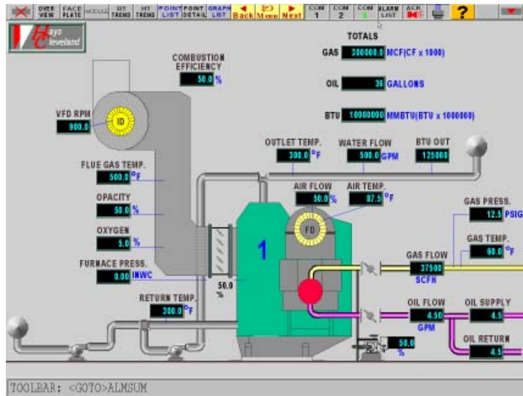
Graphical User Interface: typical SCADA screens. Above, BOILER OPERATION OVERVIEW . Below, COMBUSTION EFFICIENCY .
