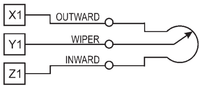
Feedback Potentiometer (Optional)
