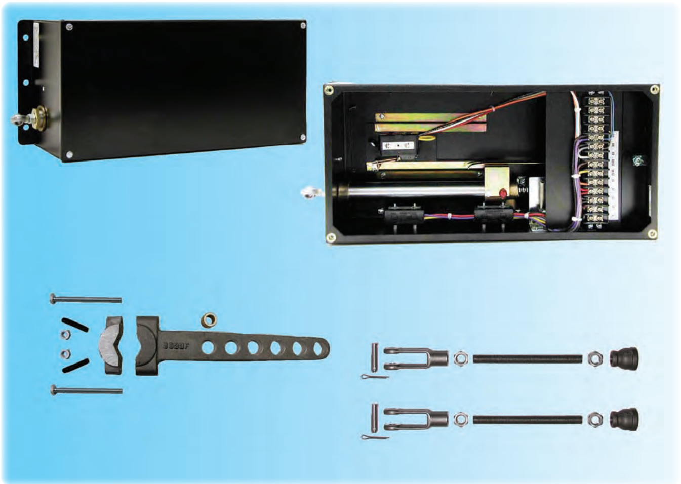
Photographs 1 & 2, top: Hays Cleveland Series F-09140 Linear Actuators are often used in draft control applications. When a Hays Cleveland Series C-07720 Sequencing Draft Control System is used with a model F-09140 Linear Actuator, adjustable starting draft positioning and other advanced options are available. See C-07720 literature for more information.
